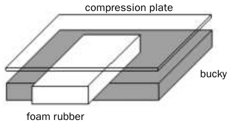
Fig. 2.5 Compression plate alignment measurement, symmetrical load
