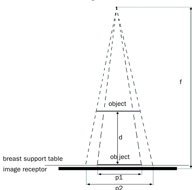
Fig. 2.2 Source-to-image distance measurement
